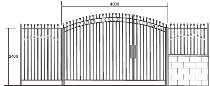
Typical Alley Gate design for Gates and Railings
